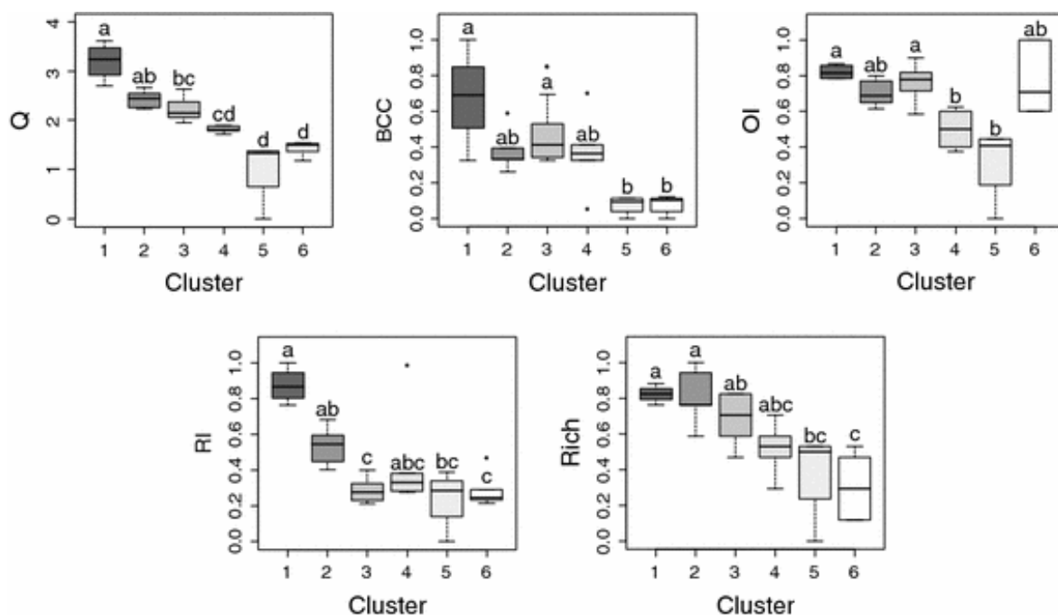
Fig. 3 Description of the classification obtained by SOM modelling. Box plots of Q , BCC, OI, RI and Rich values were plotted according to the clustering analysis, and organized along the MRPP homogeneity gradient. In each cluster, when Kruskal–Wallis tests were significant, Dunn’s post-hoc tests were conducted (the same letter means that values were not statistically different)
