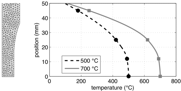
Figure 9: The temperature gradient in the dog bone specimen in a cold-grip testing machine at two temperatures [De Melo-Loseille and Lamon, 2009]
