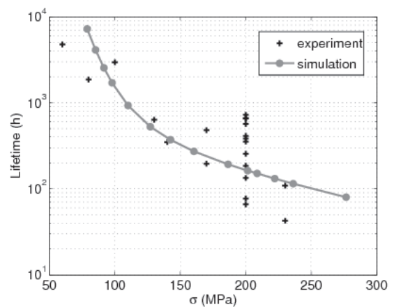
Figure 8: Comparison of the lifetime predictions between model and experiment: stress dependence at 500°C (experimental data from [Penas, 2002; Moëvus, 2007; De Melo-Loseille and Lamon, 2009])
