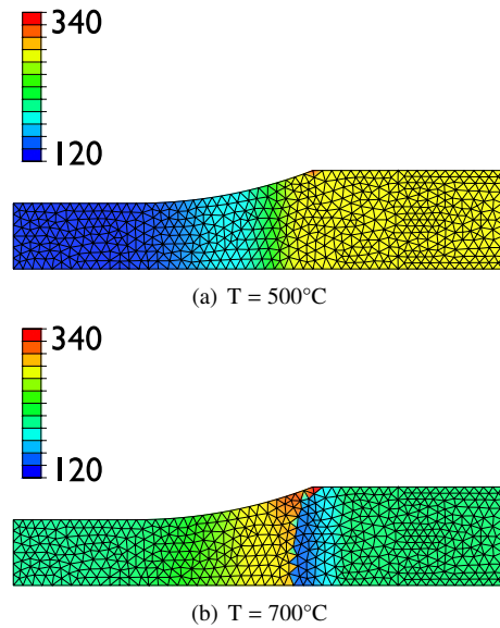
Figure 10: With a temperature gradient: the residual strength at two temperatures (200MPa loading for 278 hours)
