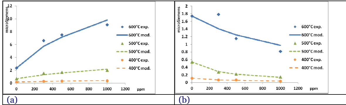
Figure 2: Variations of sensors conductance (µS) with: (a) propane (experiments and 1/2 power law models); (b) nitrogen dioxide (experiments and -1 power law models)
