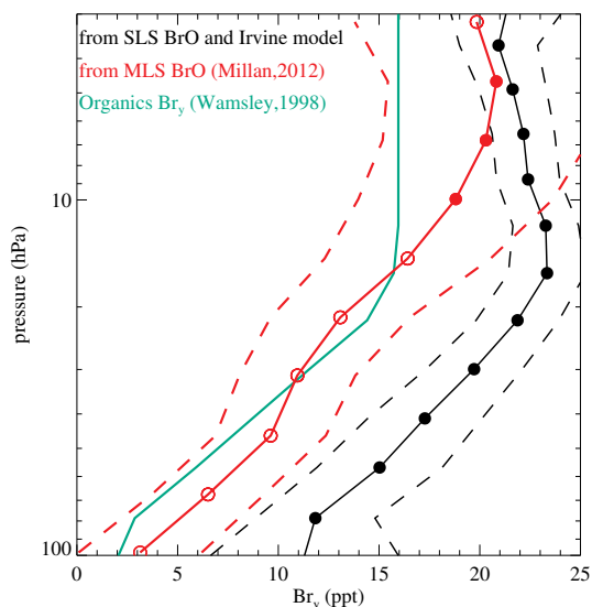
Fig. 9. Comparison of Br y mixing ratio scaled from SLS measured BrO (black) using the UC Irvine photochemical box model against Br y inferred from MLS BrO for 2005 (Millán et al., 2012). The range of scientifically useful MLS measurements (10 to 4.6 hPa) is indicated by solid circles. Uncertainties in Br y are indicated by dashed black and dashed red lines for SLS and MLS, respectively. Br y from long-lived organic gases from Wamsley et al. (1998) scaled to 16 ppt for an age-of-air of 5 yr (2006) is also plotted (cyan curve).
