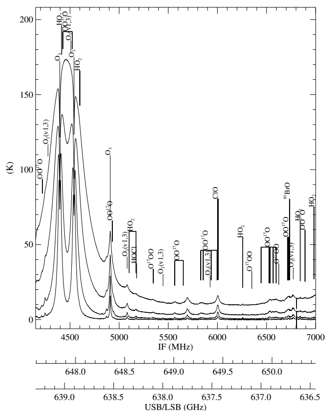
Fig. 4. Measured double-sideband emission day-time-average spectra with local oscillator frequency at 643.444 GHz. Sample spectra from the September 2011 balloon flight showing the full spectrometer bandwidth corresponding to limb tangent heights of 38, 36, 34 and 30 km. Region containing the 81 BrO lines is at the far right. Abscissa scales show intermediate frequency (IF), and upper/lower sideband frequency prior to heterodyne downconversion.
