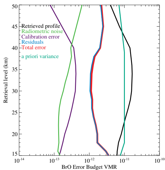
Fig. 3. The retrieval error budget showing total retrieval error and contributions from radiometric noise for flight-averaged spectra, calibration uncertainty and post-retrieval residuals compared with the a priori covariance and retrieved profile.
