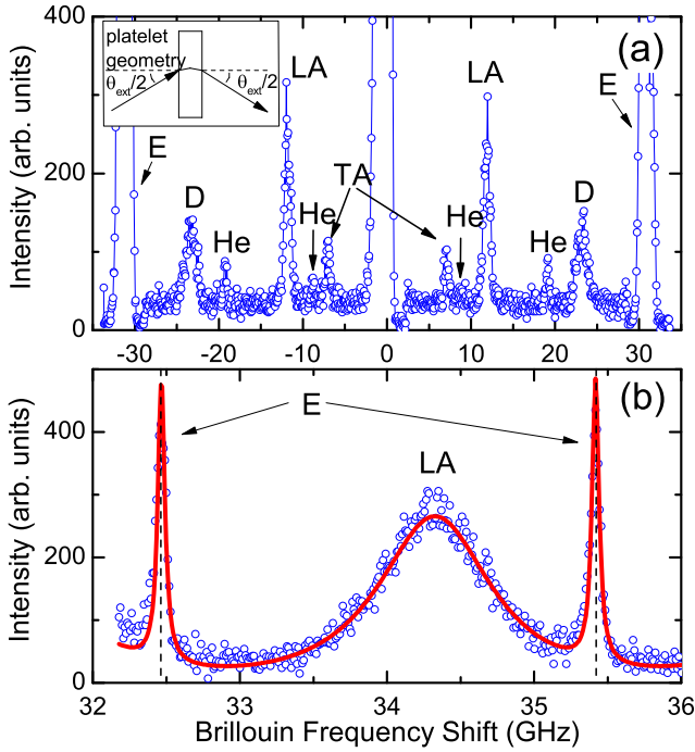
FIG. 1. (Color online) (a) Brillouin spectrum at 3.4 GPa for v -SiO 2 in He, obtained with the Sandercock spectrometer. The platelet geometry shown in the inset is used. As usual, lines emitted by He (noted He in the figure) and by the diamond anvils (D) are observed in addition to the elastic lines (E) and to the transverse and longitudinal Brillouin lines of v -SiO 2 (TA and LA respectively). (b) Brillouin spectrum of the LA modes of v -SiO 2 at 3.4 GPa measured with the high-resolution spectrometer in the backscattering geometry. The two dashed lines locate the periodically transmitted elastic peaks. The red line is a fit to the data.
