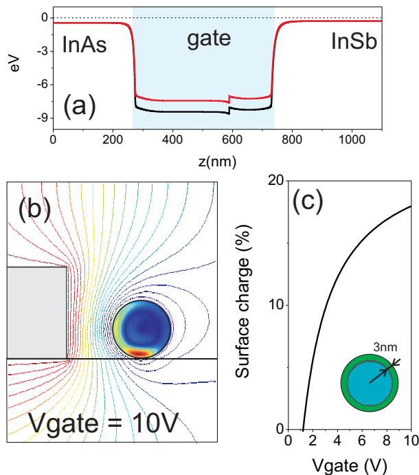
FIG. 3. (a): Schematic of the 1D band line-up of the InAs/InSb FET for a 10V gate bias (Schrödinger-Poisson). The zone in which the gate is expected to have more effect is highlighted; note that it extends very far from the junction region. (b): Charge density and isopotential lines simulated, for a 2D Poisson toy-model, for an applied gate bias of 10 V. (c): The percent of charge localized in the 3nm-outermost nanowire shell as a function of the lateral gate bias.
