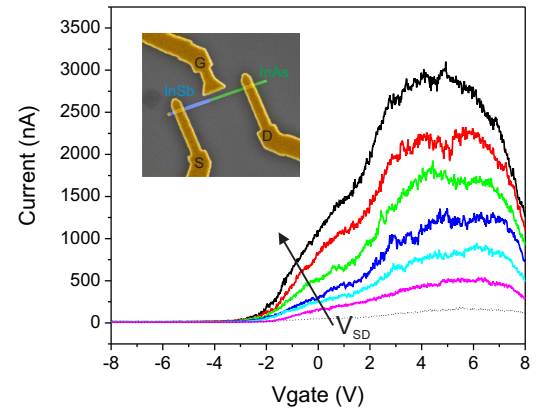
FIG. 1. I_{SD} - V_{gate} at different source-drain voltages, from 10 to 60 mV. In the inset a SEM image of the contacted wire is shown. The two arms of the log-periodic antenna realized through e-beam lithography are respectively connected to source (S) and gate (G) electrodes, while the current is measured through the drain (D) one.
