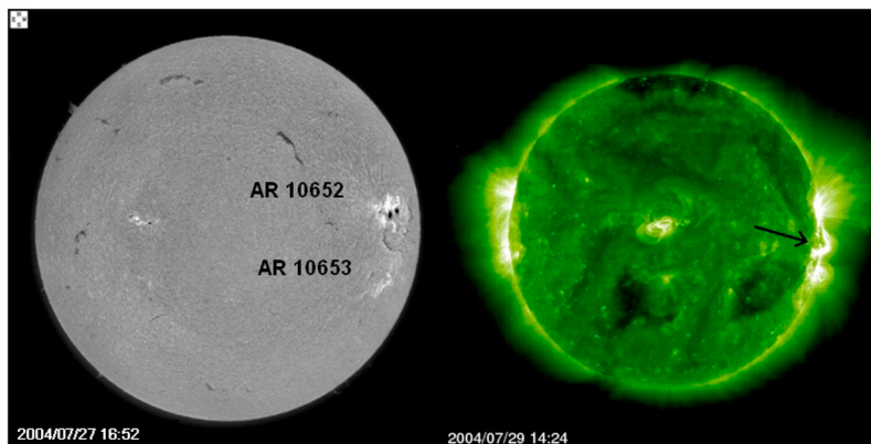
Figure 3. (left) H\alpha image obtained at Big Bear Solar Observatory showing the two ARs and the filament between them 2 days before its eruption. (right) EIT image in 195 Å after flare maximum showing the formation of interconnecting loops between AR 10652 and 10653 (pointed by an arrow).
