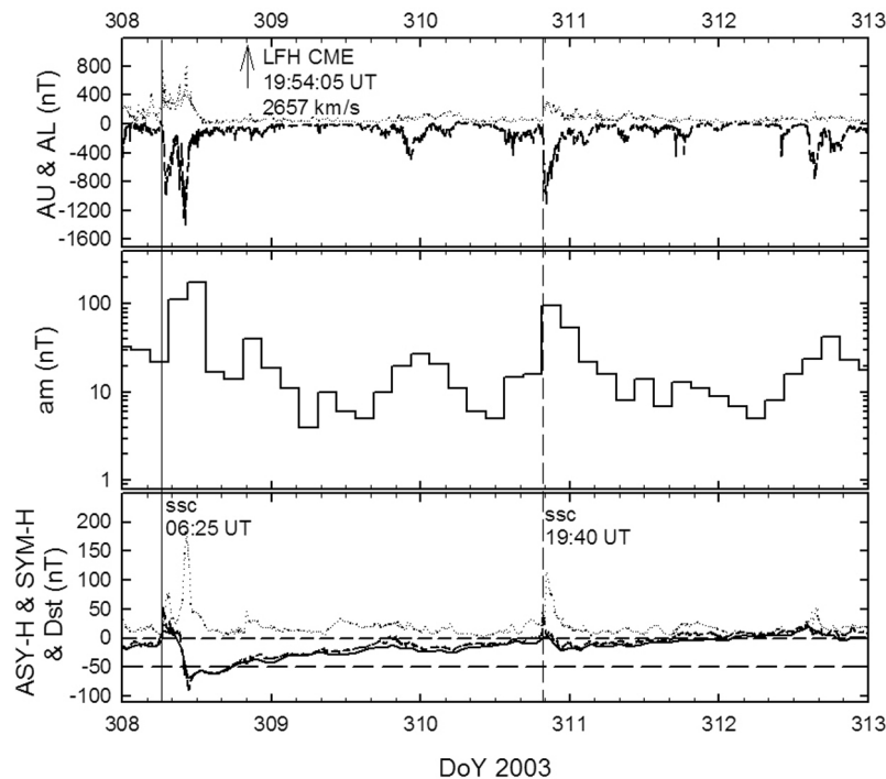
Figure 5. Geomagnetic indices for the time period 4–8 November 2003. The format is the same as that of Figure 4. The solid and dashed vertical lines mark the time of two storm sudden commencements (see text for details). An arrow in the top panel indicates the time of first appearance in the field of view of the LASCO/C2 coronagraph of the LFH CME on 4 November 2003.
