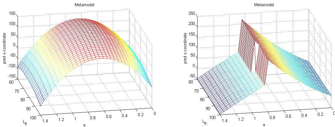
Figure 13—Combined (left) and State-Selecting (right) Quadratic Polynomial Metamodels
