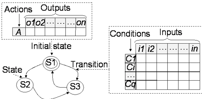
Figure 8. A finite state machine (FSM) element
