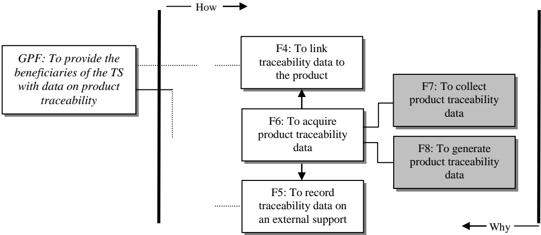
Figure 8. Identification of functions F7 and F8: To collect and to generate product traceability data
