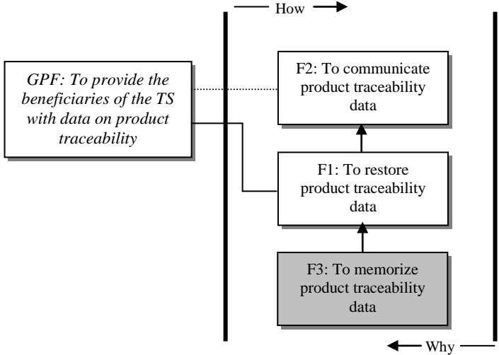
Figure 5. Identification of function F3: To memorize product traceability data
