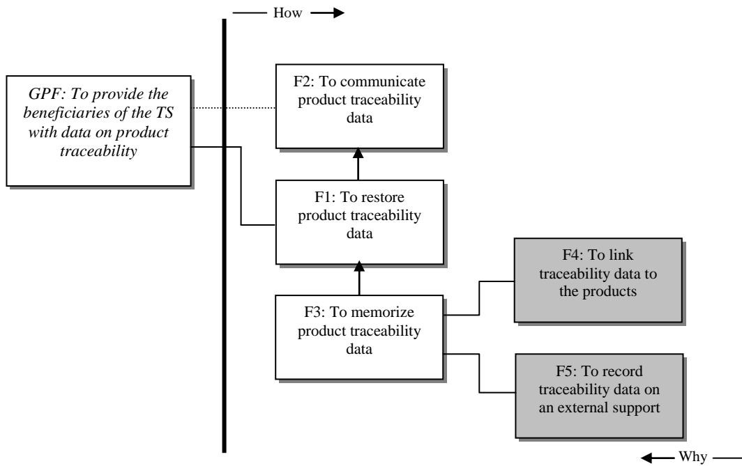
Figure 6. Identification of function F4 and function F5
