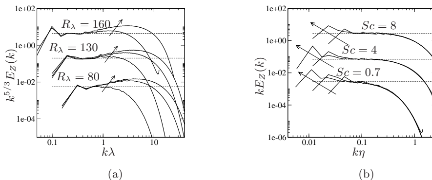
FIGURE 1. Spectrum shape at large and intermediate scales. (a) Scalar variance spectrum pre-multiplied by k^{5/3} . The wave numbers are pre-multiplied by the Taylor micro-scale, \lambda . Arrows show direction of the increasing Schmidt number, Sc . (b) Scalar variance spectrum pre-multiplied by k . The wave numbers are pre-multiplied by the Kolmogorov scale, \eta . Arrows show direction of the increasing Reynolds number, R_\lambda . Spectra are shifted for easier reading.
