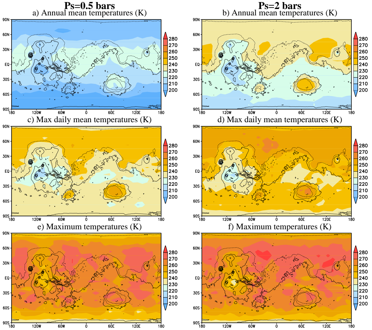
Figure 6: Surface temperatures (K) in our baseline simulations (obliquity= 25^\circ , [\text{CCN}]=10^5 \text{ kg}^{-1} , circular orbit) for mean surface pressure 0.5 bar and 2 bar. Ground albedo is as on present day Mars. Thermal inertia is set to 250 \text{ J s}^{-1/2} \text{ m}^{-2} \text{ K}^{-1} everywhere.
