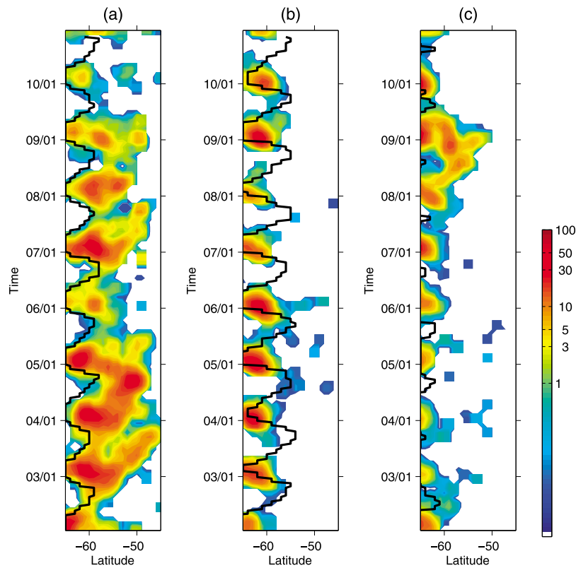
Figure 10. Time-latitude Hovmüller diagram of the monthly volume of ice (in Gt) for (a) the South Atlantic Ocean (from 70°W to 30°E), (b) the South Indian Ocean (from 30°E to 150°E) and (c) the South Pacific Ocean (from 150°E to 70°W). The thick black line represents the maximum latitude of the sea ice extent within the basin estimated from the AMSR-E sea ice data. The color scale is logarithmic.
