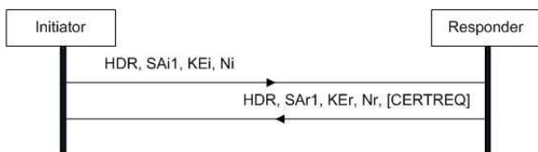
Fig. 2. IKE_SA_INIT exchange
