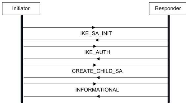
Fig. 1. IKEv2 exchanges
