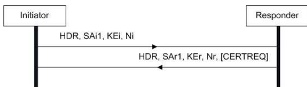
Fig. 2. IKE_SA_INIT exchange
