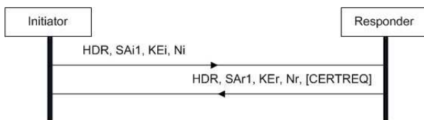
Fig. 2. IKE_SA_INIT exchange
