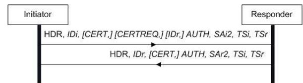
Fig. 3. IKE_AUTH exchange
