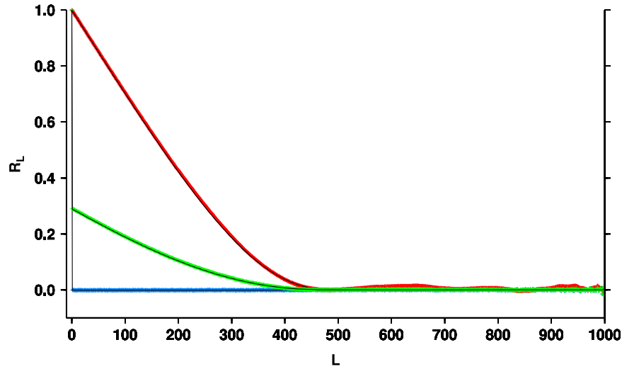
Figure B1. The autocorrelation functions R_L as a function of lag L corresponding to the three cases shown in Figure A1, except here the intermediate case uses T = 200 days. The colored plus symbols are computed with E[\gamma_L] , E[\gamma_L^b] , and E[\gamma_L^e] from an ensemble average of equations (B1), (B4), and (B5), respectively, using 3000 sample time series, while the black curves are computed with E[\gamma_L] , E[\gamma_L^b] , and E[\gamma_L^e] directly from equations (B2), (B6), and (B7), respectively.
