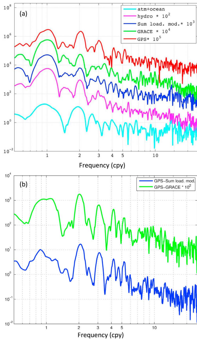
Figure 6. Stacked Lomb-Scargle normalized periodograms [Press et al., 1992] of the vertical deformations estimated at the six AMMA GPS stations by: (i) ocean and atmosphere models (MOG2D and ECMWF models – cyan curve), (ii) hydrologic model (GLDAS model – magenta curve), (iii) the sum of models (blue curve), (iv) GRACE (green curve), and (v) GPS height residuals (red curve). All the data sets are reduced to a common temporal sampling over the 2005–2008 period. The unit of the x-axis is number of cycles per year (cpy).
