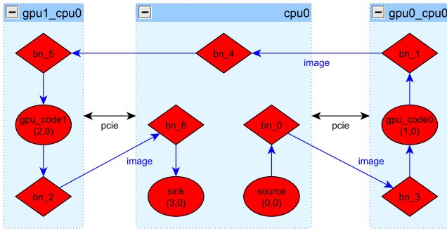
Fig. 19: Granulometry implementation graph.
