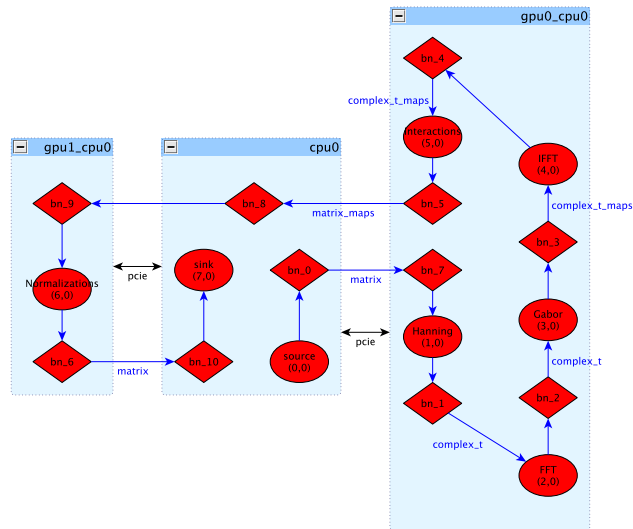
Fig. 24: Saliency implementation graph.
