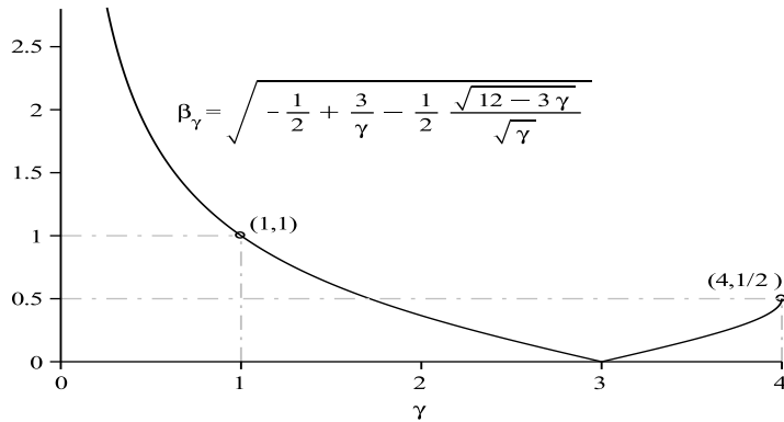
FIGURE 2.1. The plot of \beta_\gamma
