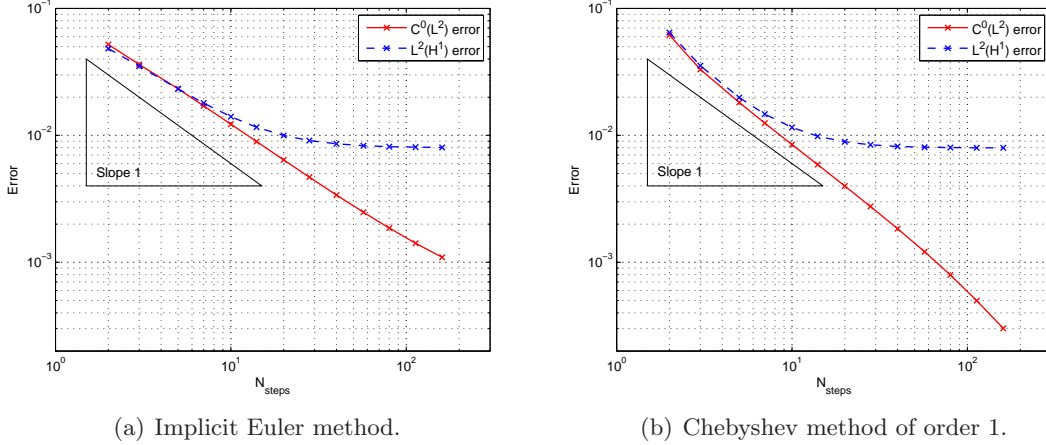
Figure 1: Linear problem (94)-(97). e_{C^0(L^2),T} error (solid lines) and e_{L^2(H^1),T} error (dashed lines) versus the number N_{steps} of timesteps. Fine macro and micro meshes ( N_{macro} = N_{micro} = 128 ).
