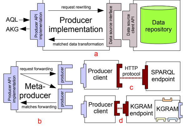
Figure 5. KGRAM Producers. Top: regular data source producer. Bottom left: meta-producer. Bottom right: producer towards remote data sources.
