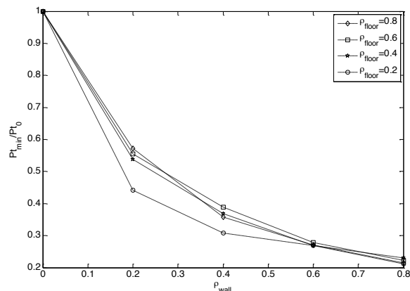
Figure 2. Ratio of power required to ensure a P_{out}=10^{-3} for BER_0=10^{-9}
