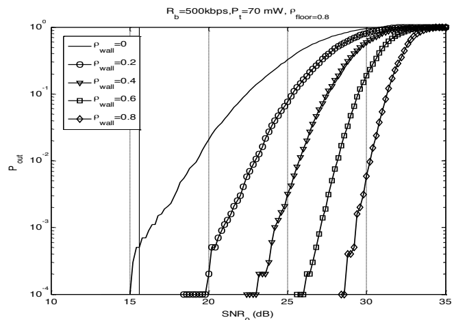
Figure 1. Impact of walls on the outage probability performances
