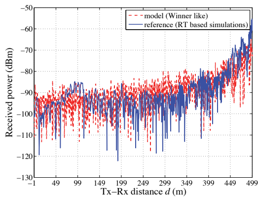
Figure 7. Received power obtained with the model and the 3D ray tracing tool versus the distance in the tunnel
