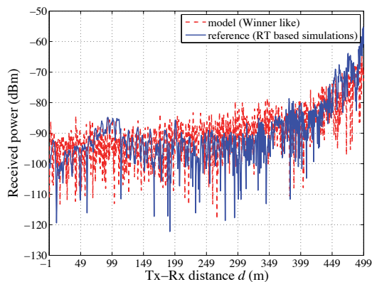
Figure 7. Received power obtained with the model and the 3D ray tracing tool versus the distance in the tunnel
