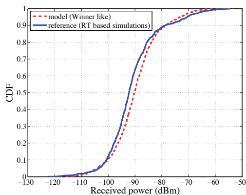
Figure 8. Cumulative Distribution Function (CDF) of the received power obtained with the model and the ray-tracing based simulation results
