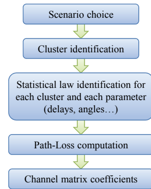
Figure 1. Followed methodology
