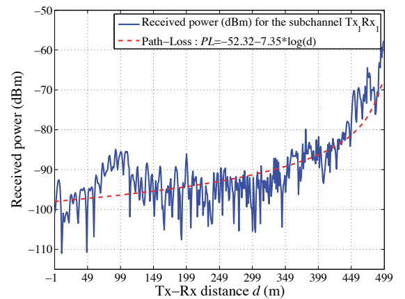
Figure 4. Received power for one SISO link versus transmitter-receiver distance
