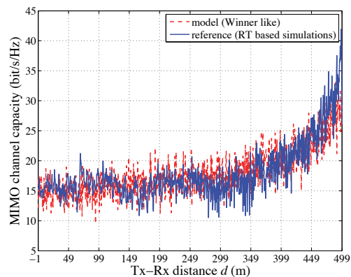
Figure 5. 4x4 MIMO channel capacity versus the distance in the tunnel computed using (x) with the two models
