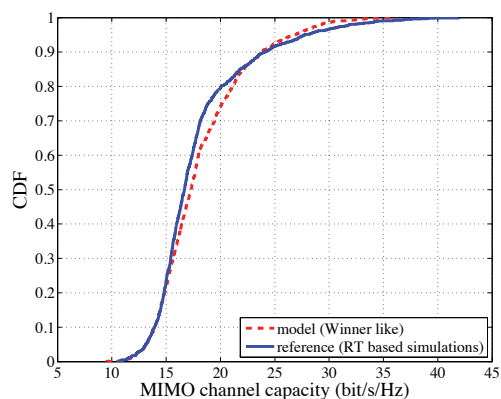
Figure 6. Cumulative Distribution Function of the 4x4 MIMO channel capacity from the channel model and the ray-tracing based simulation results
