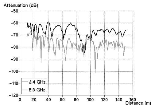
Figure 4.5 : Results for Tunnel C 2.4 GHz - 5.8 GHz
