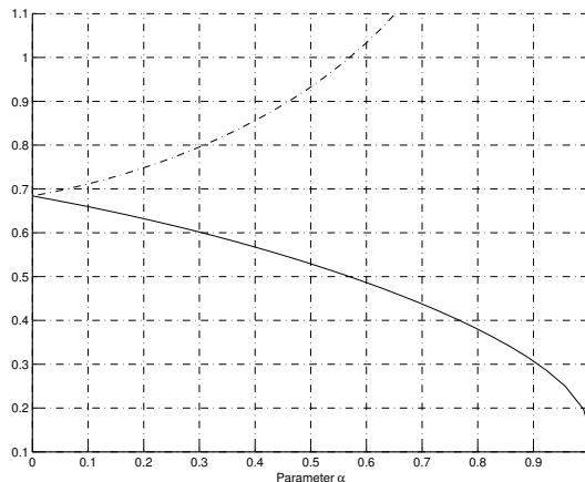
Fig. 2. Normalized ECRBs achieved by the optimal \mathbf{V} array, as a function of parameter \alpha . Solid (dash-dotted) line refers to the normalized ECRB for the angle of interest (resp. on the other angle), i.e. (18) [resp. (23)].
