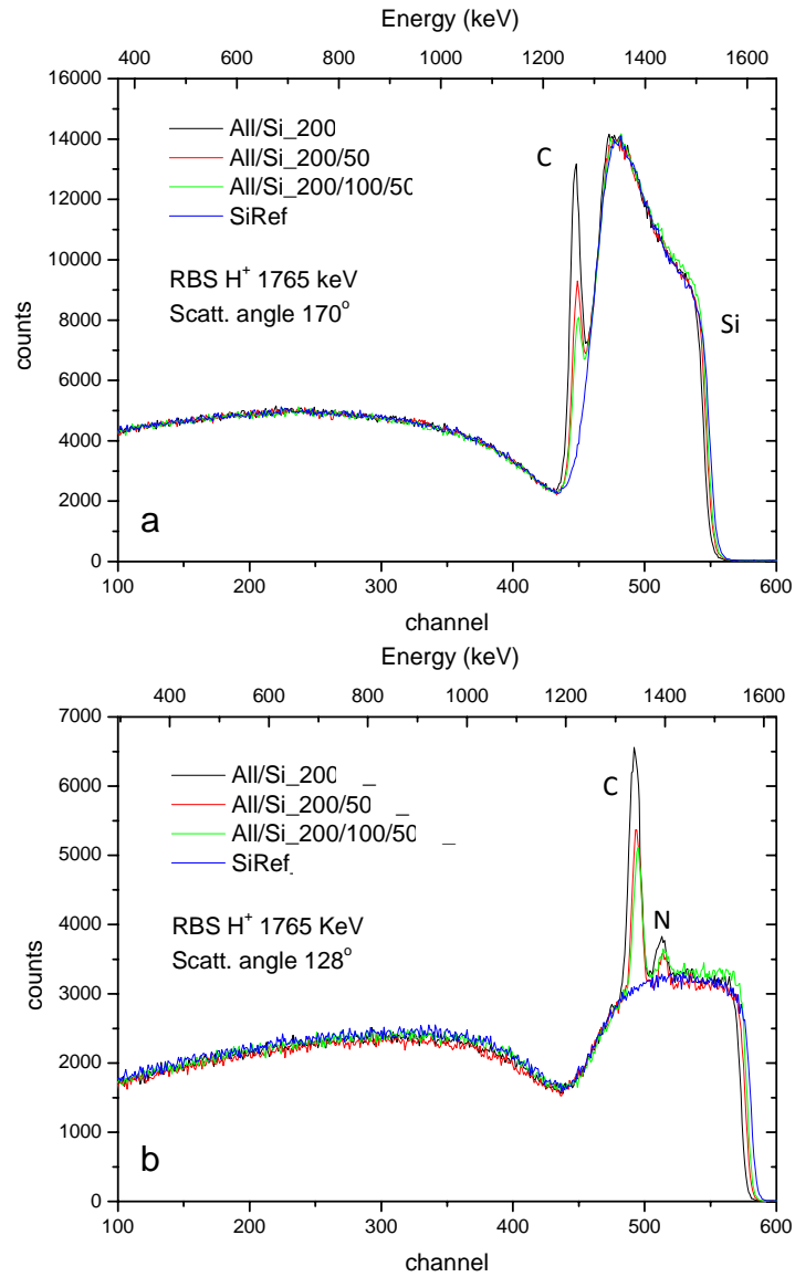
Figure 4: RBS analysis of Al/Si layers grown in gradual plasma power softening conditions measured with 1.765 MeV H^+ : a) experimental spectra at 170^\circ scattering angle, b) experimental spectra at 128^\circ scattering angle.
