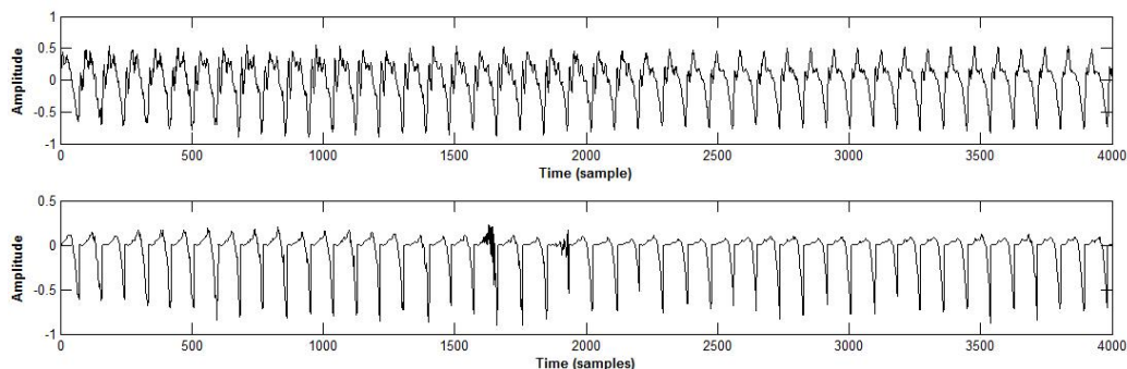
Figure 9: Top panel : A segment of voiced speech (diphone / am /) uttered by a female speaker. Bottom panel : Its corresponding glottal source estimation obtained using the complex cepstrum-based decomposition. It turns out that a reliable estimation can be achieved for most of the speech frames.
