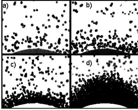
FIG. 1. Photographs of the flow around a cylinder ( R = 12 mm, h = 2 mm, glass beads of d = 0.5 mm) for different \phi_\infty = 0.004, 0.006, 0.01, \text{ and } 0.017 .
