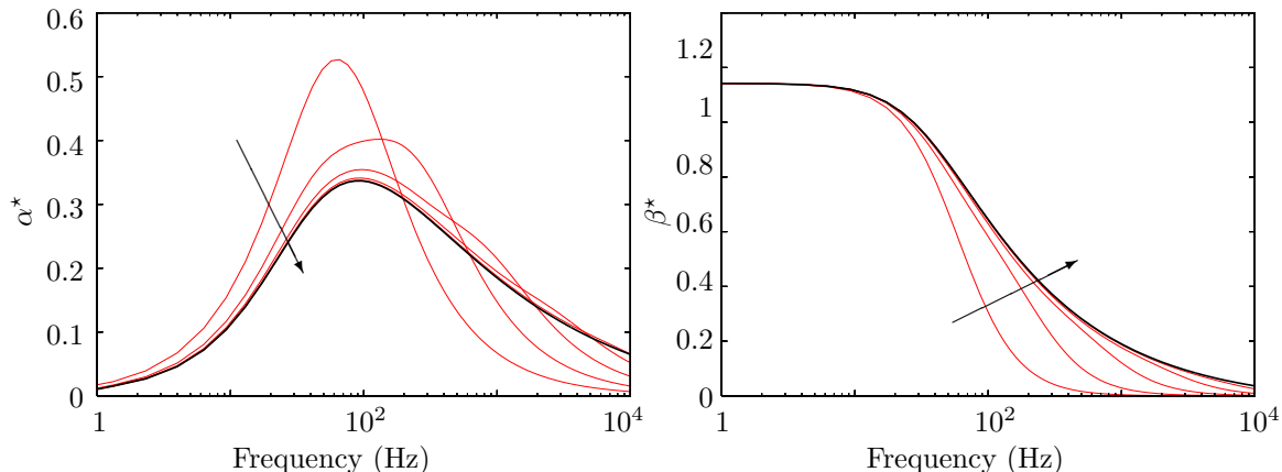
Figure 4: Convergence of the Multi-Fluid method on attenuation and dispersion of a monochromatic acoustic wave in a polydisperse window spray – Red : MF results for 1, 2, 4, 8, 16 sections; Arrow : increasing number of sections; Black : reference solution.
