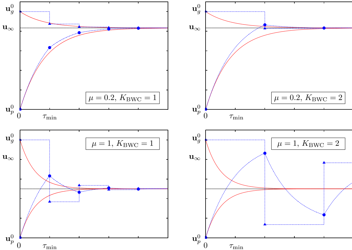
Figure 5: BWC computation of a 0D gas-particle relaxation case for different loadings and different K_{\text{BWC}} – \Delta : gas; \circ : particles; Line : exact solution for each phase.
