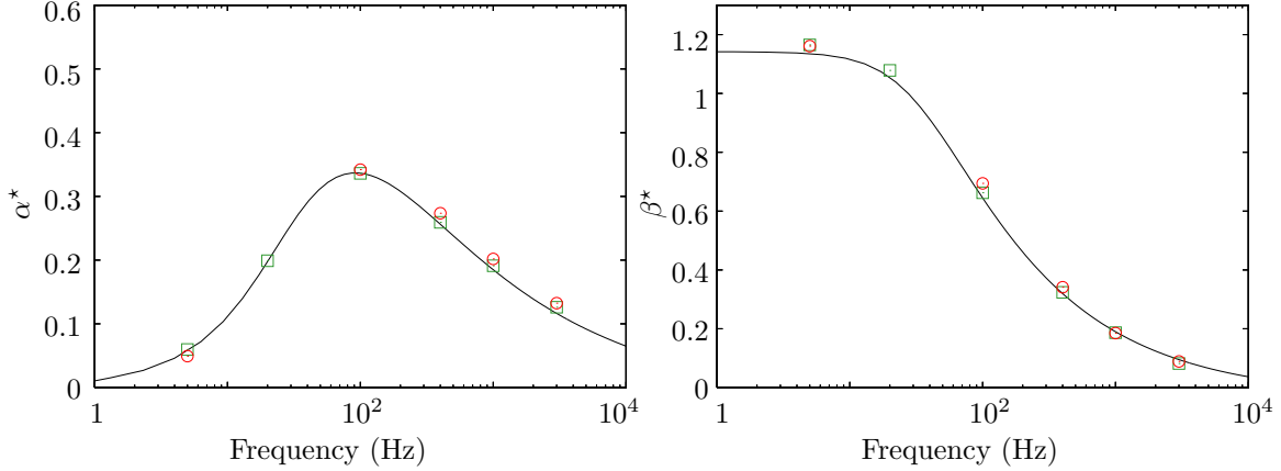
Figure 13: Attenuation and dispersion of a monochromatic acoustic wave in a polydisperse spray – Line : analytic; □ : SAP1 (ACS splitting, 10 sections); ○ : CEDRE (ACS splitting, 10 sections).
