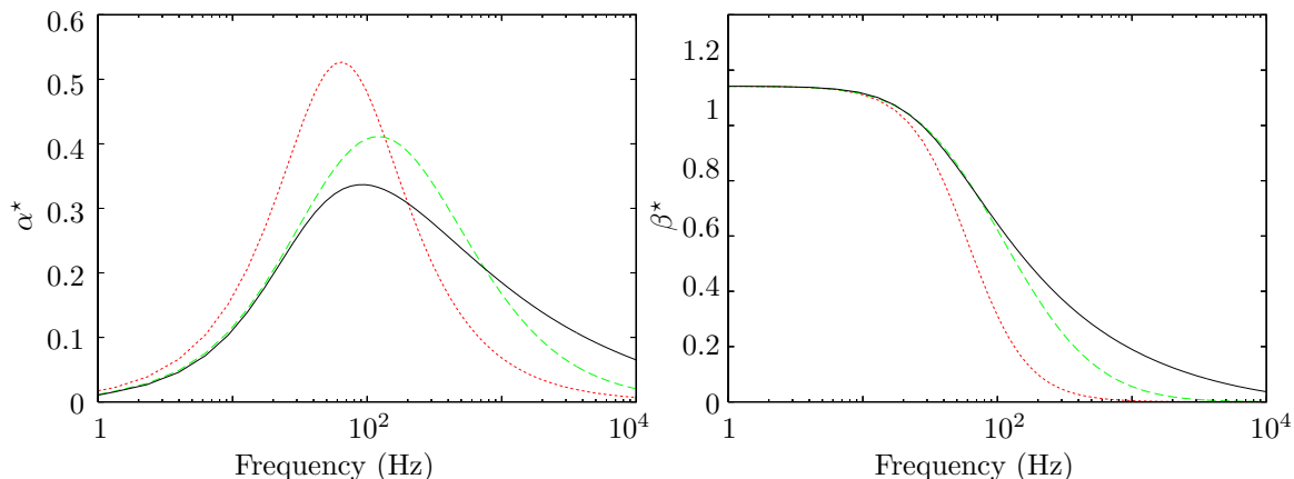
Figure 3: Attenuation \alpha^* and dispersion \beta^* of a monochromatic acoustic wave in a polydisperse spray – Dotted : Dirac size distribution (monodisperse); Dashed : lognormal size distribution; Solid : window size distribution.
