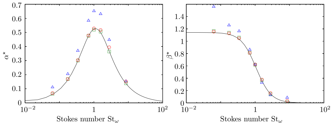
Figure 12: Attenuation and dispersion of a monochromatic acoustic wave in a monodisperse spray with \mu = 0.106 – Line : analytic; \Delta : CEDRE (BWC technique); \square : SAP1 (ACS splitting); \circ : CEDRE (ACS splitting).
