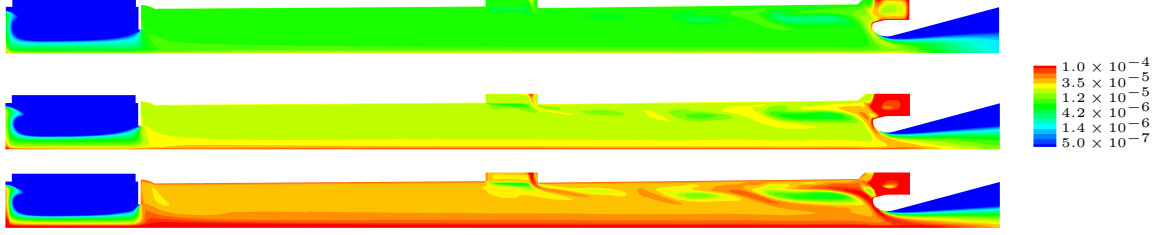
Figure 15: Instantaneous volume fraction per section in LP10 with CEDRE (MF-PEG ACS (top to bottom: S , M and L droplets)).
