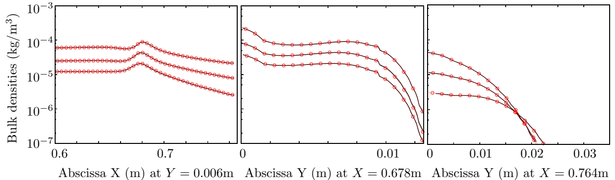
Figure 16: Droplet mass concentrations along cuts (left: cut A-A, middle: cut B-B, right: cut C-C) – Solid : MF-PEG BWC (reference); o : MF-PEG ACS.
