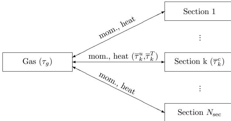
Figure 1: Gas and Multi-Fluid equation coupling and time scales of the system
