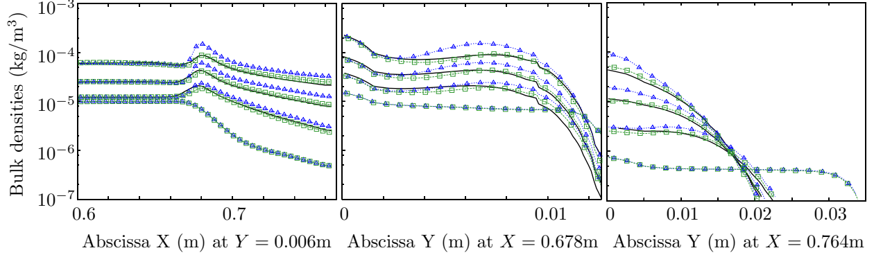
Figure 18: Droplet mass concentrations along cuts (left: cut A-A, middle: cut B-B, right: cut C-C) – Solid : MF-PEG reference (BWC); \Delta : MF BWC; \square : MF ACS.
