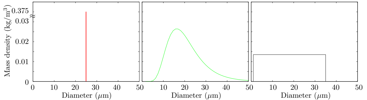
Figure 2: Different droplet size distributions with the same total bulk density – Left: Dirac size distribution (monodisperse); Middle: lognormal size distribution; Right: window size distribution.
