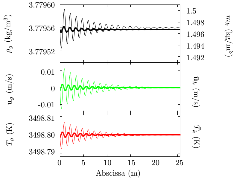
Figure 7: Propagation test case for St_\omega = 20 with \mu = 0.106 – Gas variables (thin line) and liquid variables (+) once the wave has completely penetrated
