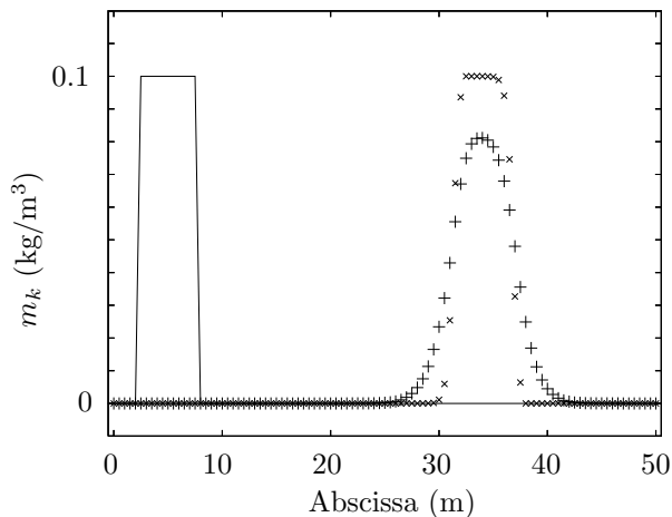
Figure 9: Convection of a liquid structure with a time step driven by acoustics (window packet convected at 30m/s, second order Bouchut scheme, SAP1 code) – + liquid transport at CFL_k = 0.081 ; \times liquid transport at CFL_k = 0.94 ; —: initial state.
