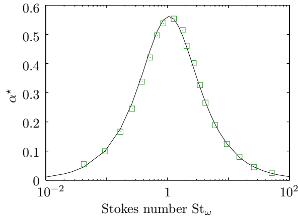
Figure 11: Attenuation of a propagative sine profile in a monodisperse spray with \mu = 0.106 and with ensemble motion – Line : analytic; □ : SAP1 with ACS, K_g = 0.9 .
