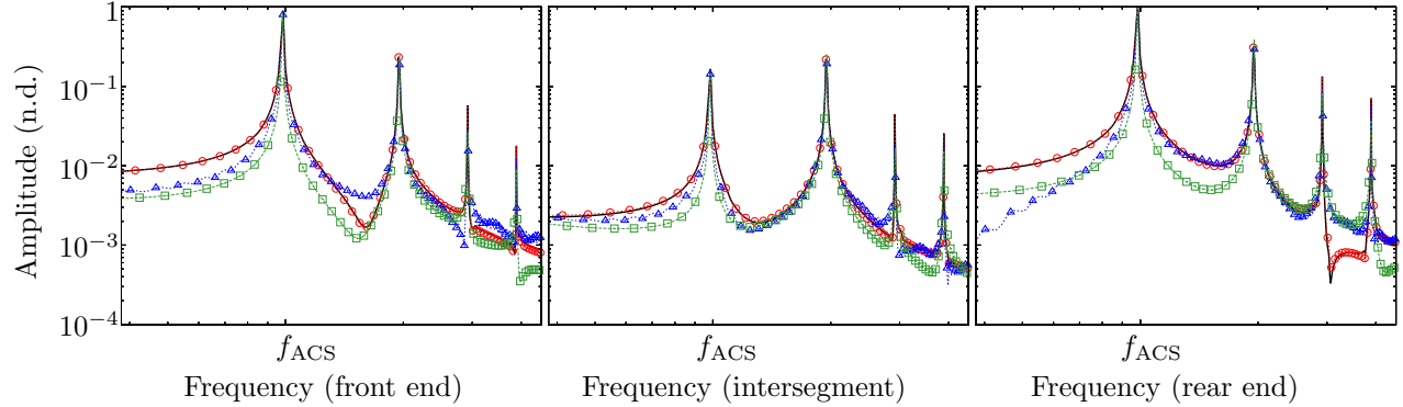
Figure 20: Spectra of pressure signal non dimensioned by the ACS highest peak – Left: front-end sensor (1); Middle: middle sensor (2); Right: rear-end sensor (3) – Solid : MF-PEG BWC (reference); o : MF-PEG ACS; Δ : MF BWC; □ : MF ACS.
