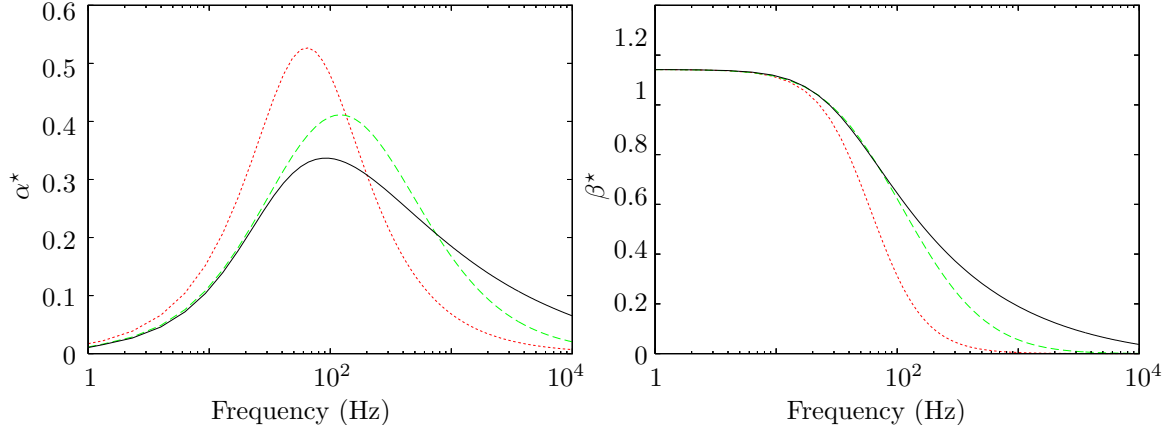
Figure 3: Attenuation \alpha^* and dispersion \beta^* of a monochromatic acoustic wave in a polydisperse spray – Dotted: Dirac size distribution (monodisperse); Dashed: lognormal size distribution; Solid: window size distribution.
