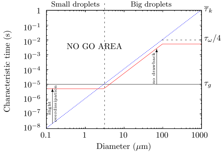
Figure 6: Typical acoustics time scales plotted versus droplet diameter – Black : gas time \tau_g ; Dotted : typical droplet relaxation time \tau_{\min} (BWC timestep must be smaller); Red : prescribed acoustic time step \Delta t_a for ACS with K_g = K_p = 0.5 .
