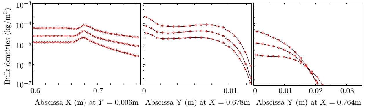
Figure 16: Droplet mass concentrations along cuts (left: cut A-A, middle: cut B-B, right: cut C-C) – Solid : MF-PEG BWC (reference); o : MF-PEG ACS.
