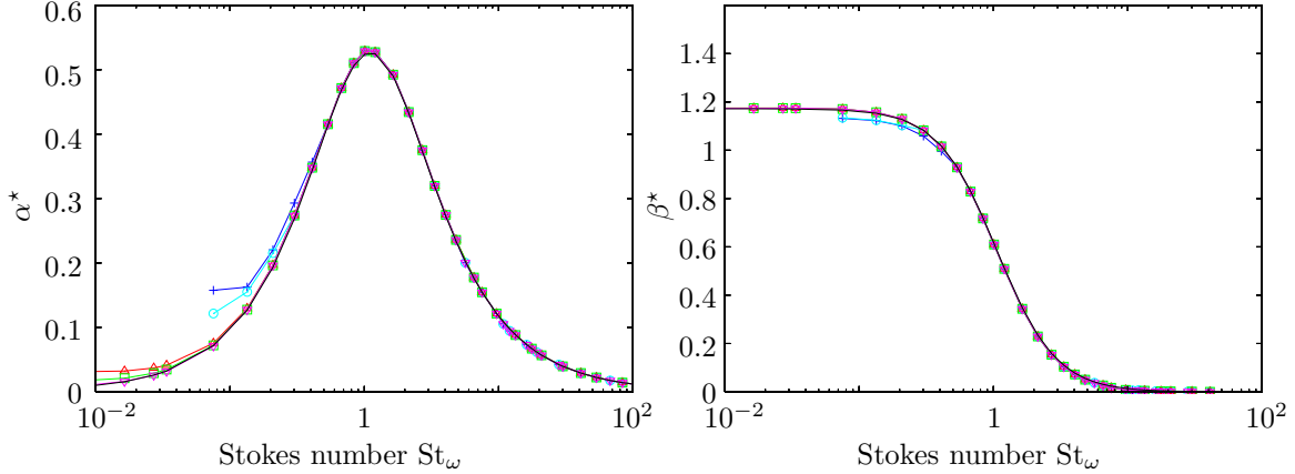
Figure 8: Attenuation and dispersion of a monochromatic wave in a monodisperse spray with \mu = 0.106 for different coupling time steps (SAP1 code, K_p = 0.25 ) – Line : analytic; + : K_g = 2 ; o : K_g = 1 ; Δ : K_g = 0.9 ; □ : K_g = 0.5 ; ▽ : K_g = 0.2 .
