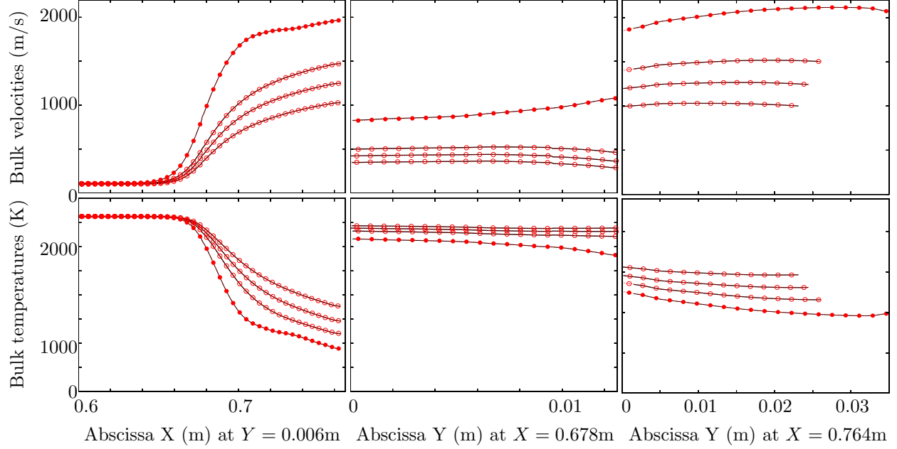
Figure 17: Velocities and temperatures along cuts (left: cut A-A, middle: cut B-B, right: cut C-C) – Solid : MF-PEG BWC (reference); \circ : MF-PEG ACS – Empty symbols: disperse phase; Full symbols: gas.
