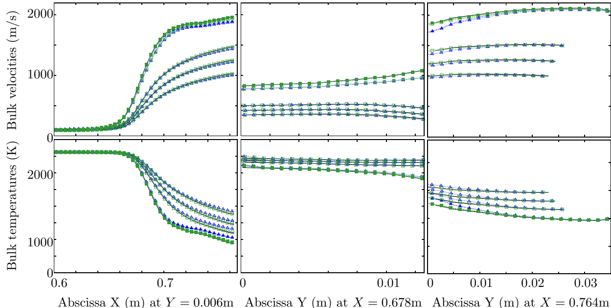
Figure 19: Velocities and temperatures along cuts (left: cut A-A, middle: cut B-B, right: cut C-C) – Solid : MF-PEG reference (BWC); \triangle : MF BWC; \square : MF ACS – Empty symbols: disperse phase; Full symbols: gas.
