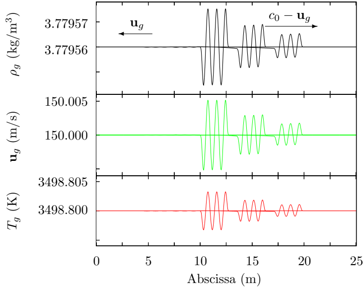
Figure 10: Convective test case in a spray with \mu = 0.106 – Gas variables at three different times (Initial state: centered 3-period sine profile)
