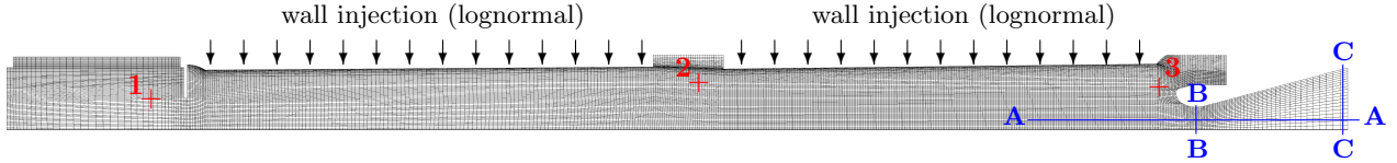
Figure 14: Deformed-structured 27,000 cell mesh of the LP10 geometry ( Arrow : injection; Line : cut; + : pressure sensor).
