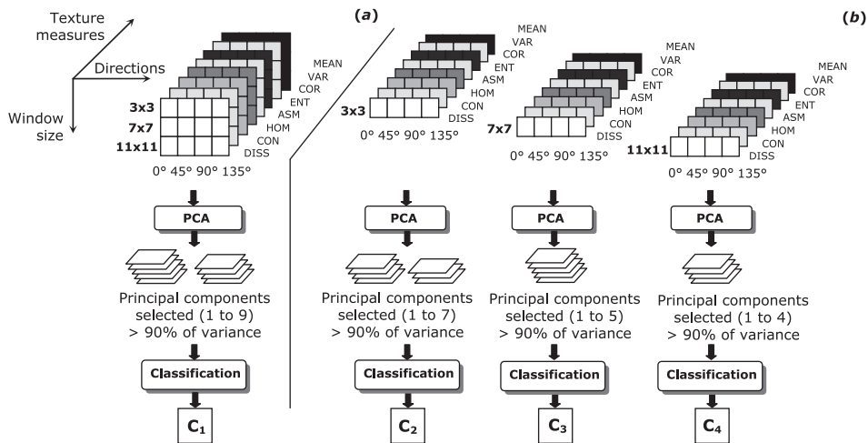
Figure 2. The classification strategies tested to assess the usefulness of adding texture. Each cell of the matrix represents one texture image related to one texture measure (DISS, dissimilarity; CON, contrast; HOM, homogeneity; ASM, angular second moment; ENT, entropy; COR, correlation; VAR, variance; MEAN), one window size and one direction. In the first strategy (a), a principal component analysis (PCA) was computed using all the texture variables including all the window sizes and directions. In the second strategy (b), a PCA was applied on each set of texture variables related to one window size and including all directions.
