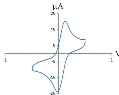
Fig. 2 Cyclic voltammogram of the title compounds in DMF at 0.1 V s −1 at a glassy carbon electrode restricted to the reversible system.
