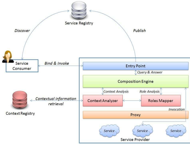
Figure 4. Global architecture.
