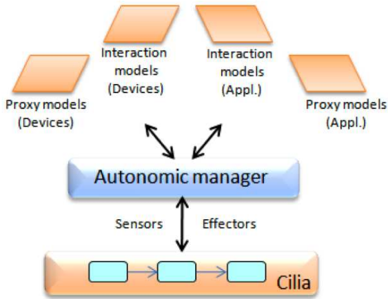
Figure 4. DynaMo model-based autonomic manager.
