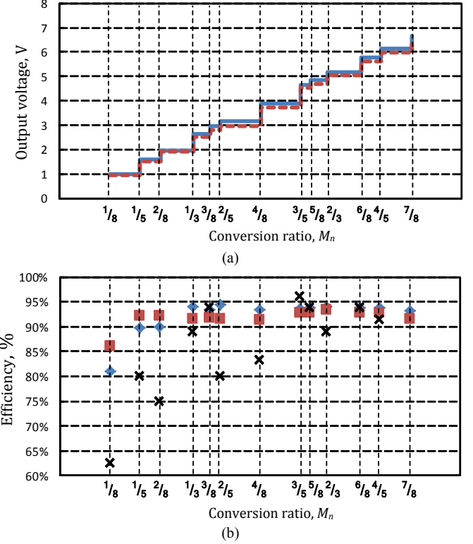
Fig. 7: The output voltage (a) and efficiency (b) of the experimental SCC. Diamonds: R_o=300\Omega . Squares: R_o=100\Omega . The curve of the higher output voltage in (a) is for R_o=300\Omega , while the one of the lower output voltage is for R_o=100\Omega . The points marked by "X" in (b) are estimates of minimum efficiency of a regulated version of proposed SCC in between target voltages.
