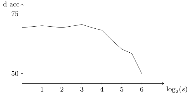
Fig. 1. Evolution of d-acc for data set glass
