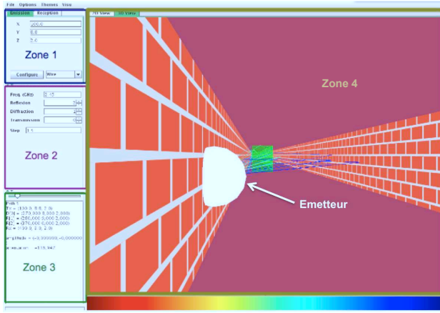
Fig. 2. Radio propagation simulator interface
