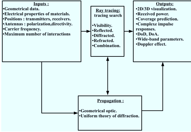
Fig. 1. Synoptic of the radio propagation simulator
