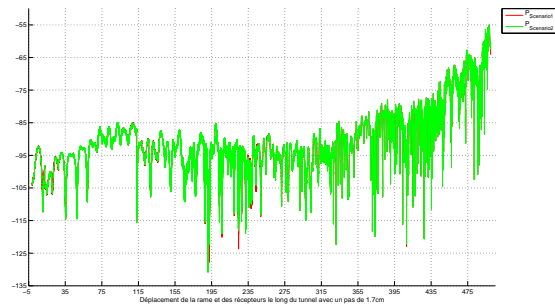
Fig. 9. Evolution of total received power for different environments modeling
