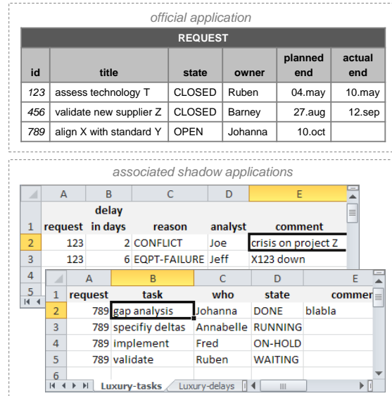
Figure 1. Example of fictional official database and associated shadow application data.
