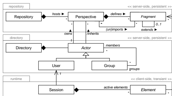
Figure 2. Meta-model of Perspective-centric architecture.
