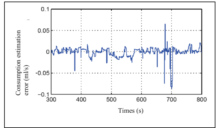
Figure 1. Estimation error of the fuel consumption.
