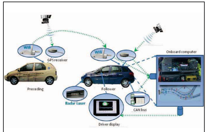
Figure 7. Vehicles equipment.
