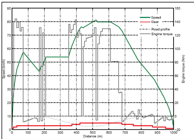
Figure 2. Optimal speed profiles and gear ratio versus weighed coeff. Q_j .
