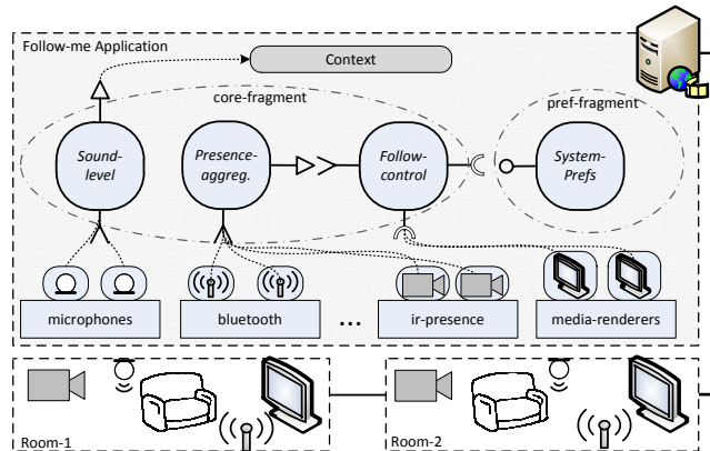
Figure 4: Scenario Follow-me
