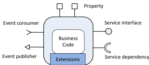
Figure 2: Component Model
