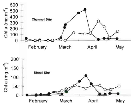
Fig. 5. Time series of phytoplankton biomass (as chl a ) at the channel site and shoal site. Each panel shows the changing concentrations of chl a in the upper sediments (O) and the integrated chl a concentration in the overlying water column (●)
