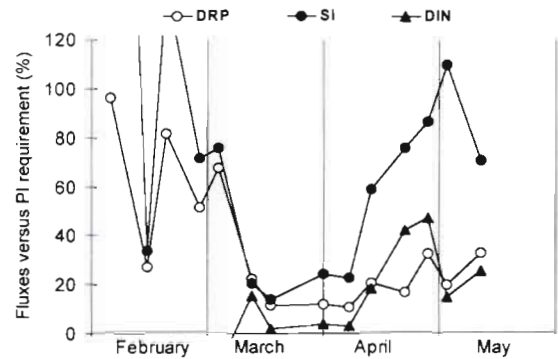
Fig. 8. Time series of the contribution of benthic nutrient fluxes to the requirement for phytoplankton primary production, estimated for the entire South San Francisco Bay (see 'Benthic supply versus phytoplankton demand for nutrients')
