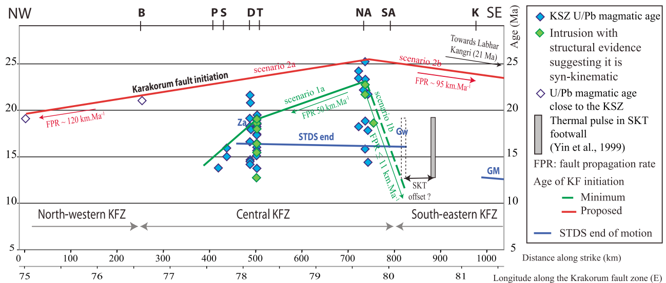
Figure 12. Age constraints on the onset and propagation of the KFZ. U/Pb ages are plotted along the strike of the fault. Green diamonds indicate syntectonic granitoids (Leloup et al. [2011], Reichardt et al. [2010], this study, Valli et al. [2008], and Wang et al. [2011]). Data and corresponding references are reported in Text S6. K, Kailas; NA, North Ayilari; SA, South Ayilari; T, Tangtse; D, Darbuk; S, Satti; P, Panamik; B, Baltoro; GM, Gurla Mandata; SKT, South Kailas Thrust. The green line delineates the minimum age for the KFZ initiation (scenario 1a), assuming that the oldest synkinematic granitoids (green framed diamonds) date the fault initiation. The red line delineates the maximum age for the KFZ initiation (scenario 2), assuming all Miocene granitoids (blue diamonds) are synkinematic. The dashed green line delineates the KFZ propagation to the SE if the SKT was active until \sim 13 Ma and if it predates the KFZ (scenario 1b). In each case, the corresponding fault propagation rates (FPR) are indicated below the line. See section 6.2 for details. The blue line delineates the timing of South Tibetan detachment system (STDS) end of motion, according to Leloup et al. [2010]. Modified from Leloup et al. [2011].
