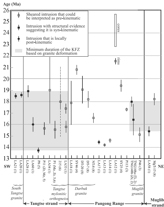
Figure 8. Summary of ages and relationships with strike-slip shearing of the magmatic rocks in the Tangtse area. Samples are presented from (left to right) SW to the NE. All ages are for zircons, unless stated with the sample name (Zr: zircon; Ti: titanite; Mz: monazite). Numbers in bracket are key to original references: (1) This study; (2) Reichardt et al. [2010]; (3) Phillips [2004]; (4) Jain and Singh [2008]; (5) Phillips et al. [2004]; (6) Searle et al. [1998]; (7) Leloup et al. [2011]; (8) Ravikant et al. [2009]. U/Pb Magmatic bodies (granites and dykes) emplaced continuously between at least \sim 21.6 Ma (LA12) (this study) and \sim 13.7 Ma (P8) [Phillips et al. , 2004], with no visible trend in age from SW to NE. The oldest and the youngest intrusion with structural evidence for synkinematic emplacement define the minimum fields for right-lateral ductile deformation (gray), see sections 5.1.2 and 5.1.3 for details.
