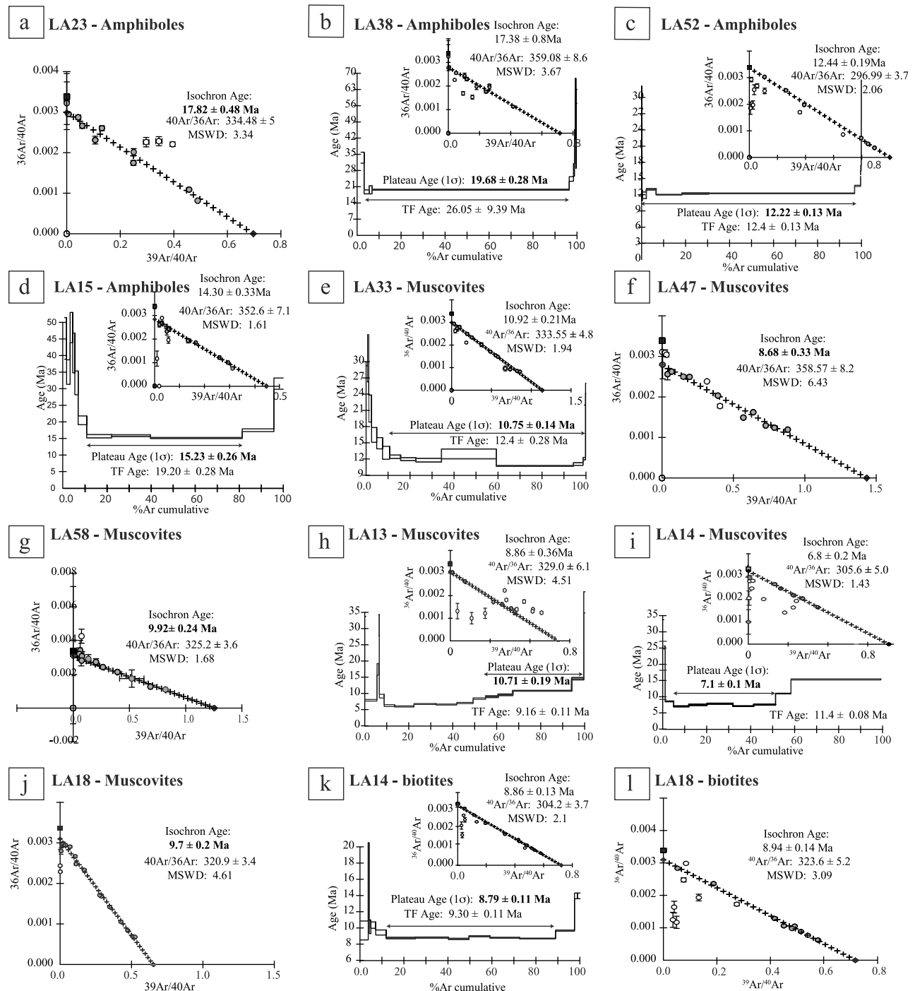
Figure 4. Ar/Ar dating. Results are summarized in Table 3. The age spectra and/or the inverse isochron plots are given. When the plateau age is significant, it is retained and otherwise, the inverse isochron age is retained. In age spectra plots, steps taken into account for the plateau age calculations are designated by a double arrow. In the inverse isochron plots steps taken in the regression calculation are in gray. Figures 4a to 4d show amphiboles, Figures 4e to 4j show muscovites, and Figures 4k to 4x show biotites. Samples: (a) LA23; (b) LA38; (c) LA52; (d) LA15; (e) LA33; (f) LA47; (g) LA58; (h) LA13; (i) LA14; (j) LA18; (k) LA14; (l) LA18; (m) LA21; (n) LA28; (o) LA38; (p) LA33; (q) LA34; (r) LA47; (s) LA48; (t) LA52; (u) LA58; (v) LA25; (w) LA12; (x) LA13.
