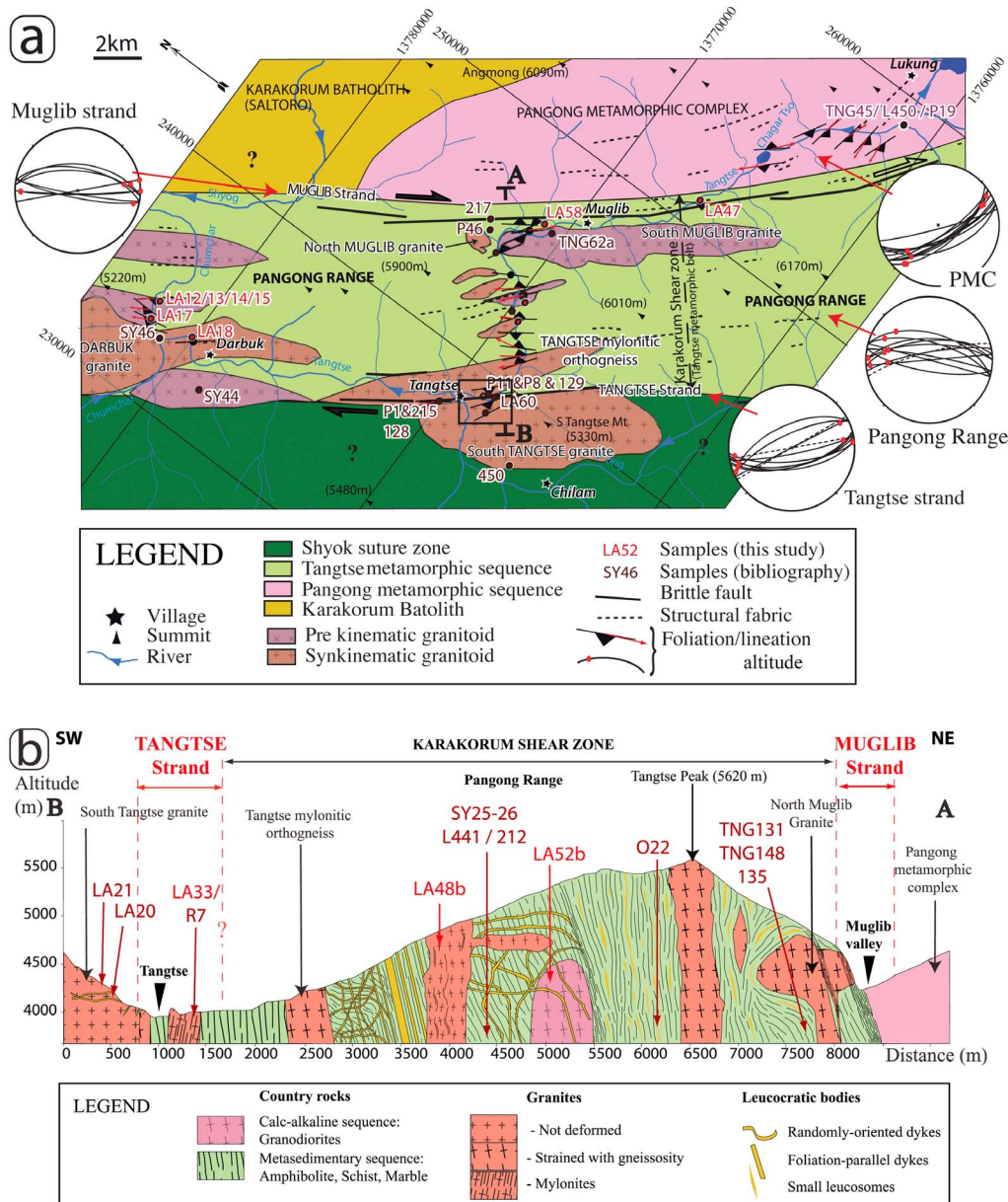
Figure 2. Structure of the KFZ in Tangtse-Darbuk zone. Most samples discussed in text are located either on a map (Figure 2a) or a section (Figure 2b). Samples from the South Tangtse granite and Tangtse strand near the Tangtse monastery are located in Figure 5. (a) Structural map drawn from field observation, satellite image interpretation, and bibliography [Phillips et al. , 2004; Reichardt et al. , 2010; Rolland et al. , 2009; Weinberg et al. , 2009]. UTM 44 projection, the black-framed zone corresponds to Figure 5a. Plots of foliations and lineations in the various units are Schmidt diagram, lower hemisphere projection. (b) Cross section along the Tangtse gorge (A-B).
