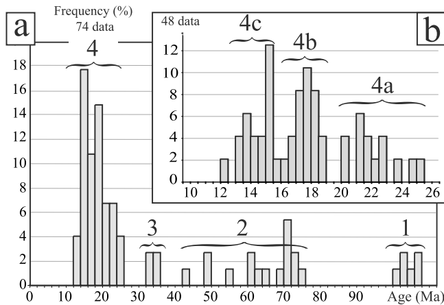
Figure 13. Population histogram of published U/Pb ages along the KFZ (a) Mesozoic and Cenozoic ages, 74 data. Paleozoic and Precambrian inherited ages have not been plotted. See Text S6 for the references. Four main magmatic events are distinguished (1, 2, 3 and 4, see section 6.1). (b) Neogene granitoids, 48 Data. Three main magmatic events are distinguished within event 4 (4a, 4b and 4c). See section 6.1 for details.
