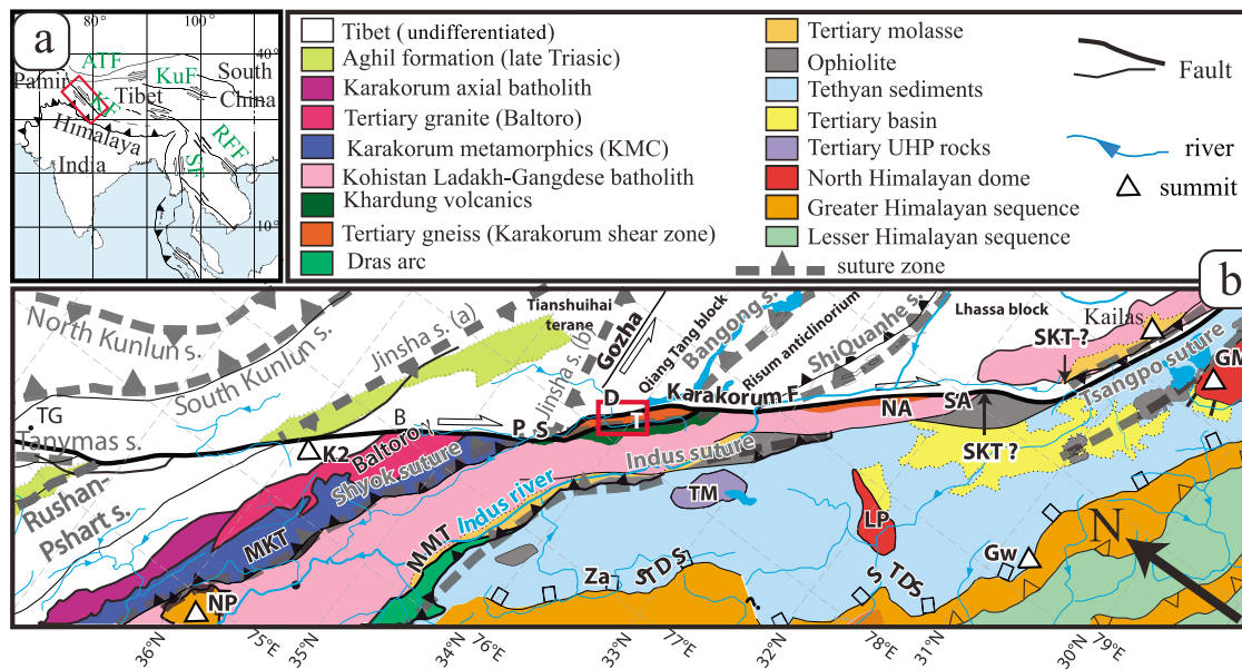
Figure 1. The Karakorum fault zone in the frame of the India - Eurasia collision. (a) Simplified structural map of the India-Eurasia collision zone. Red frame locates Figure 1b. (b) Map of the Karakorum Fault zone. SA, South Ayilari (Namru); NA, North Ayilari; T, Tangtse; D, Darbuk; S, Satti; P, Panamik; Za, Zanskar; TG, Tash Gurgan; Gw, Garwal; GM, Gurla Mandata; LP, Leo Pargil; TM, Tso Morari unit; SKT, South Kailash thrust; NP, Nanga Parbat. Red-framed area corresponds to Figure 2a. Geological units drawn from bibliography and Landsat imagery interpretation. MKT: Main Karakorum thrust corresponding to the Shyok suture zone; MMT: Main Mantle Thrust corresponding to the Indus suture zone. Modified from Leloup et al. [2011].
