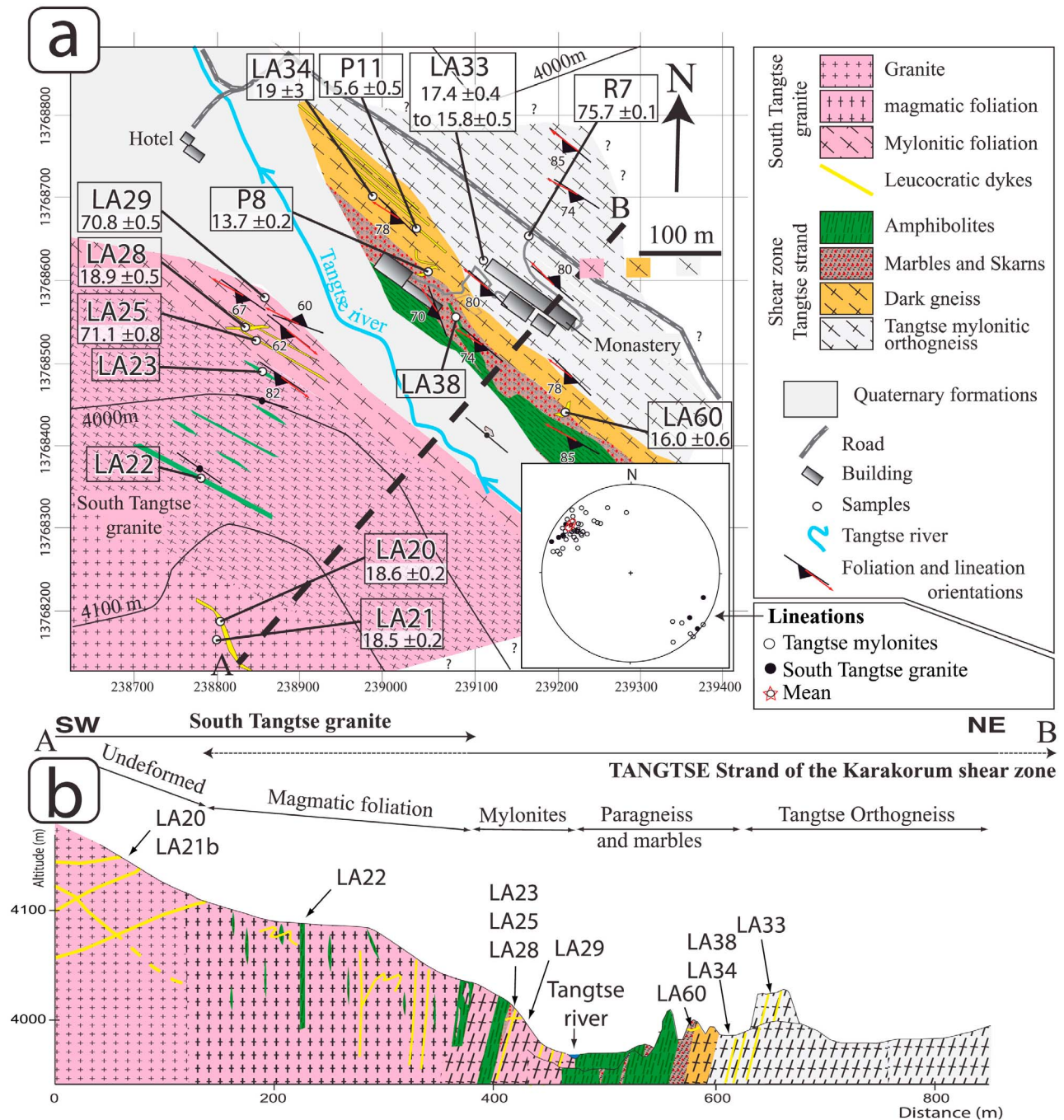
Figure 5. Map of the KSZ near the Tangtse monastery and corresponding cross-section. (a) Structural map corresponding to the black-framed zone in Figure 2a. Drawn from field observations. UTM projection (zone 44), WGS 84 ellipsoid. Samples are located, with corresponding U/Pb ages when available (Jain and Singh [2008], Leloup et al. [2011], Phillips et al. [2004], and this study). The inset is a Schmidt plot of the stretching lineations (lower hemisphere projection). The white black dashed line corresponds to the cross-section seen in Figure 5b. (b) Cross section of the Tangtse Gumpa area with samples locations. Same legend as for Figure 5a.
