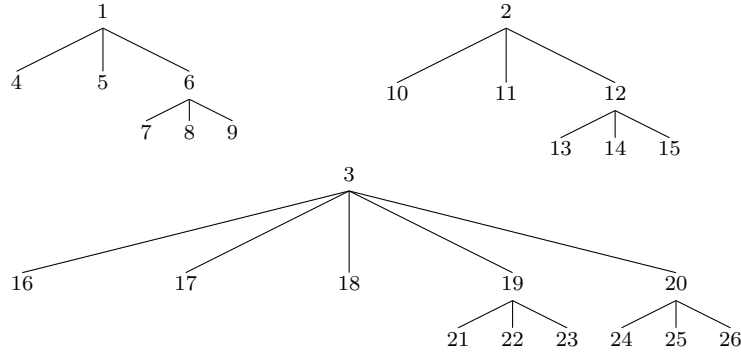
Figure 6: The relation \prec_B on the nodes of the branch in Figure 5
