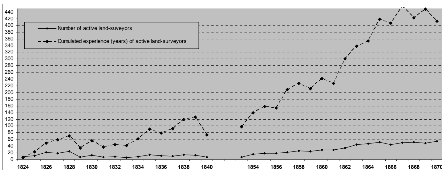
Figure 7. Temporal evolution of cumulated experience of the land-surveyors group and of the number of active land-surveyors.
