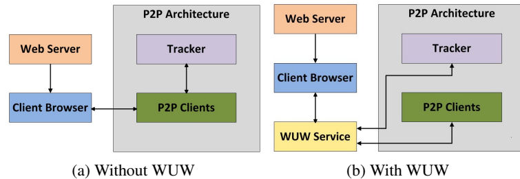
Fig. 2: Global view of the P2P-based CDN application.
