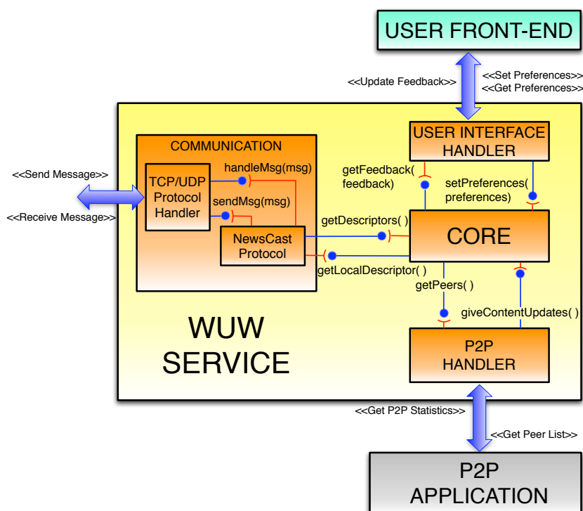
Fig. 1: WUW architecture.
