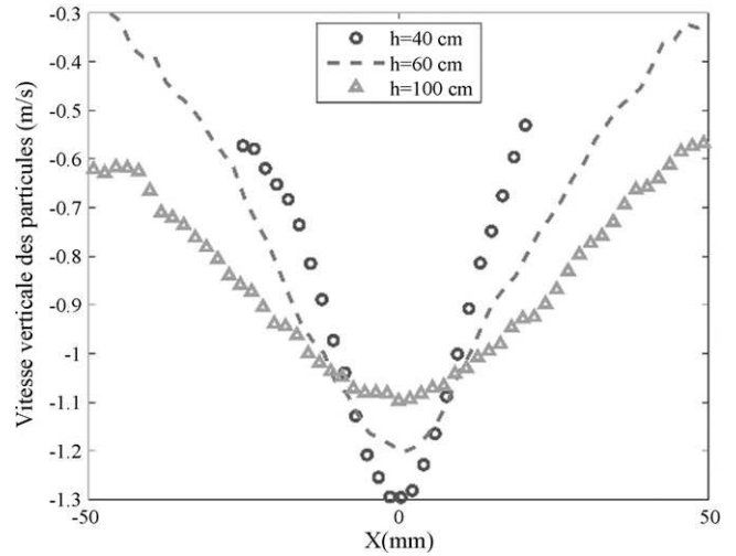
Fig. 8. Vertical particle velocity.
