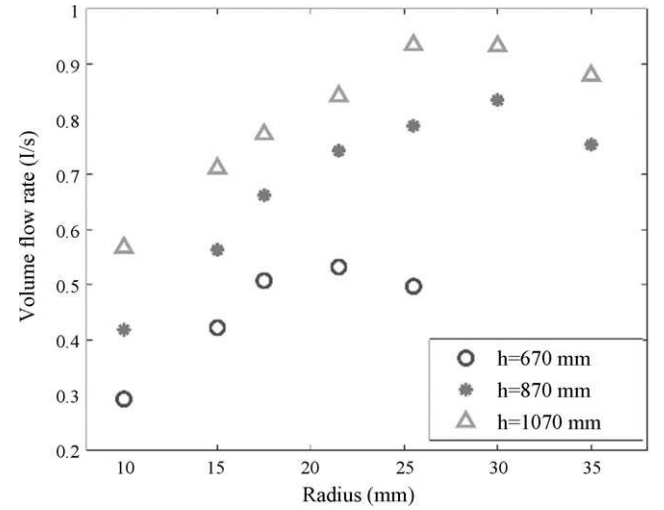
Fig. 11. Volume flow rate of entrained air.
