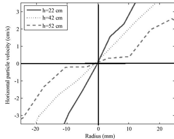
Fig. 7. Horizontal particle velocity.
