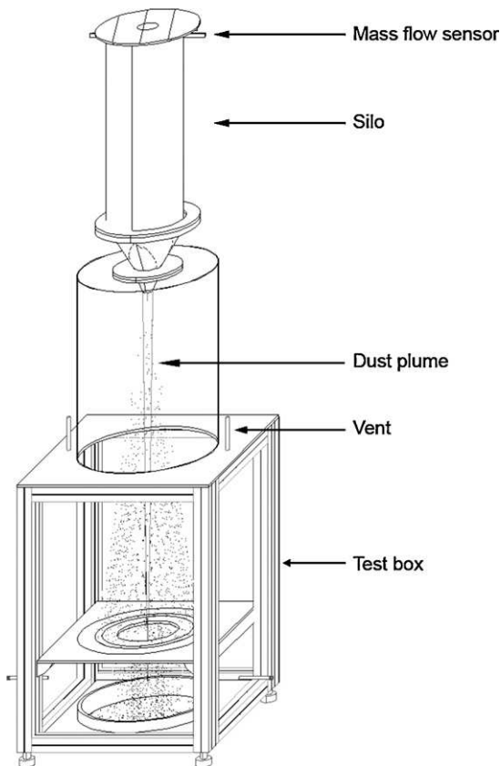
Fig. 2. Sketch of the experimental set up.
