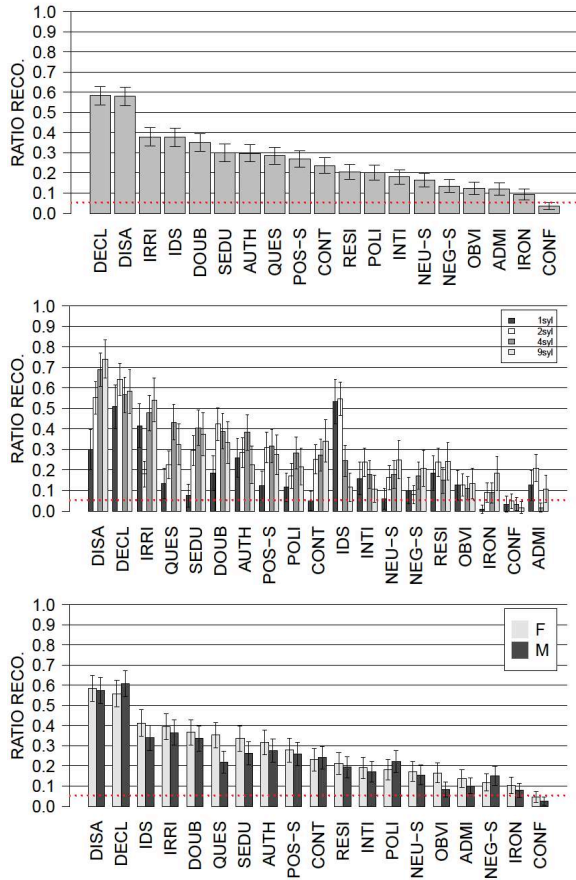
Figure 1: The mean recognition for 19 social affects: rate per attitude (top), rate per stimuli's length (middle) and rate per gender (bottom)
