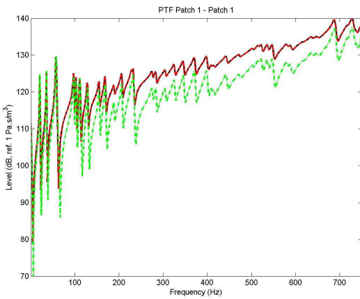
Figure 4. Comparison of three methods for estimating the input patch transfer function: dash-dotted line, modal superposition without residual shapes; dash line, modal superposition with residual shapes; solid line, direct FEM results.
