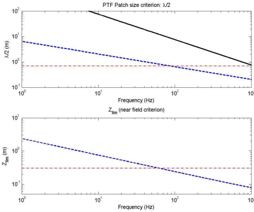
Figure 2. Patch size criteria \lambda/2 (upper) for the fluid medium (black) and for the plate structure (blue). Z_{lim} parameter defined by Eq. (10) (lower).
