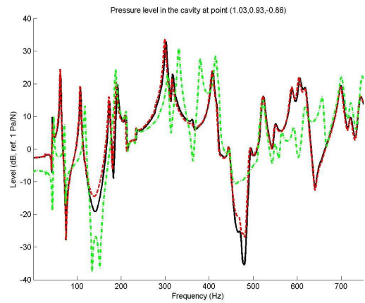
Figure 5. Comparison between three calculations of the pressure level in the cavity of the test case: dash-dotted line, PTF results using modal superposition without residual shapes; dash line, PTF results using modal superposition taking the residual shapes into account; solid line, direct FEM results.
