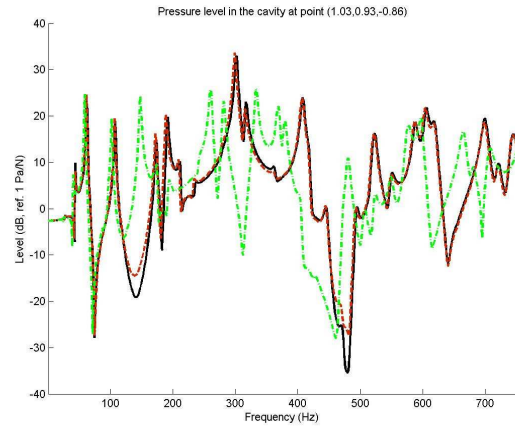
Figure 3. Comparison of the pressure level inside the cavity for three calculations: red line, PTF results with the first substructuring; green line, PTF results with the second substructuring; black line, direct FEM results (reference).
