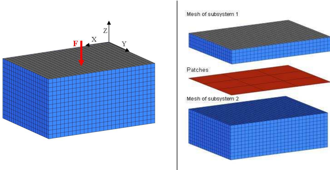
Figure 1. Structure-Cavity problem and PTF substructuring.
