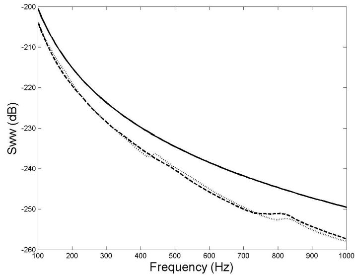
Figure 3: Frequency spectrum of the plate displacement at (0,0) for a TBL excitation. without stiffeners (solid line); stiffener spacing: 1m (dash line); stiffener spacing: 1.35 m (dotted line)
