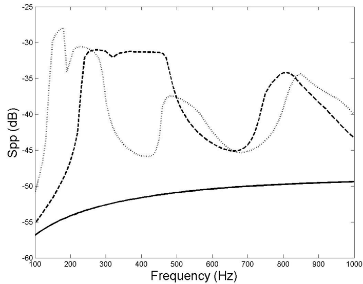
Figure 4: Frequency spectrum of the radiated pressure at (0,0,100m) for a TBL excitation. without stiffeners (solid line); stiffener spacing: 1m (dash line); stiffener spacing: 1.35 m (dotted line)
