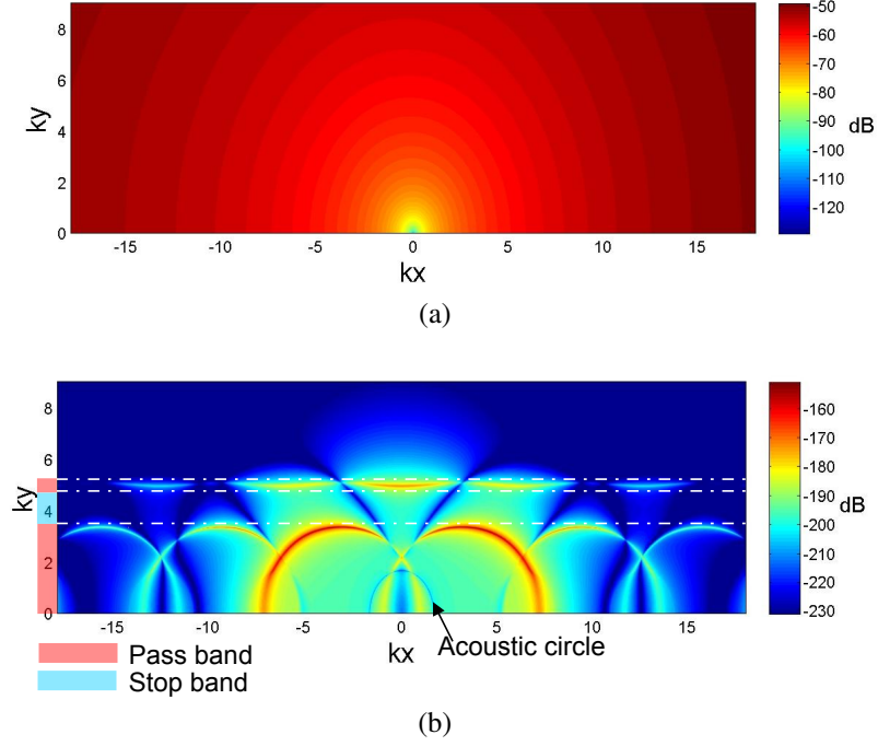
Figure 2: (2a), Wavenumber spectrum of the TBL wall pressure \Phi_{pp}(k_x, k_y) at 400 Hz (Chase model). (2b), Wavenumber spectrum of the plate displacement \tilde{W}(k_x, k_y) at 400 Hz for a force excitation on a rib. Stiffener spacing: 1m.
