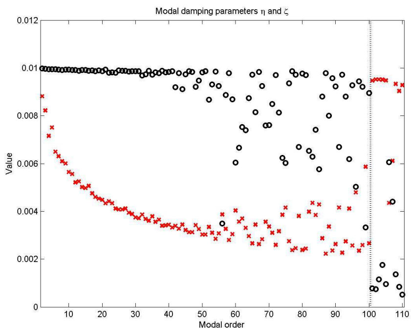
Figure 9. Values of damping parameters \eta and \zeta for each modal order: crosses, values for \eta ; circle, values for \zeta . Vertical dotted line, splitting between the 100 normal modes and the 10 residual shapes.
